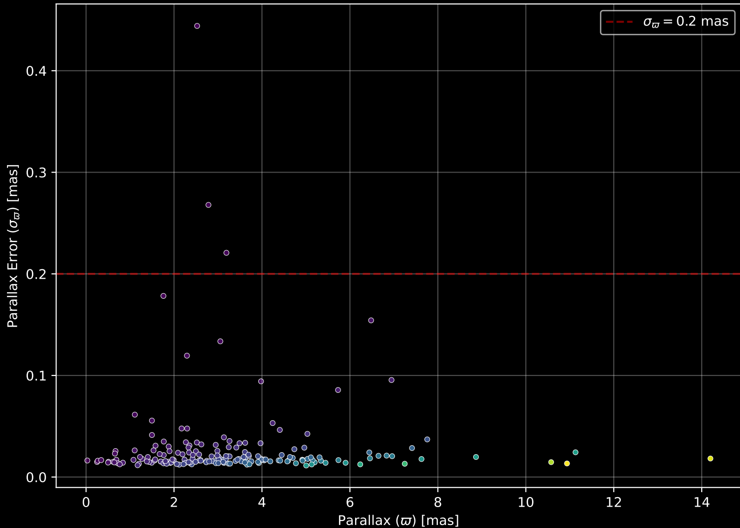
APOGEE DR17 Field: [165+62_MGA] Parallax Quality (n= 184)
