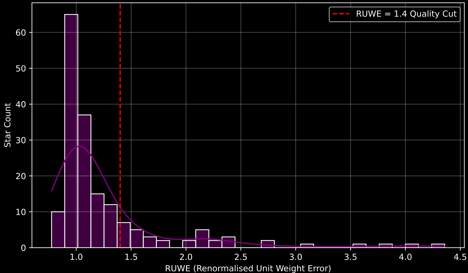
GAPOGEE DR17 Field [165+62_MGA] RUWE Distribution (n= 175)
