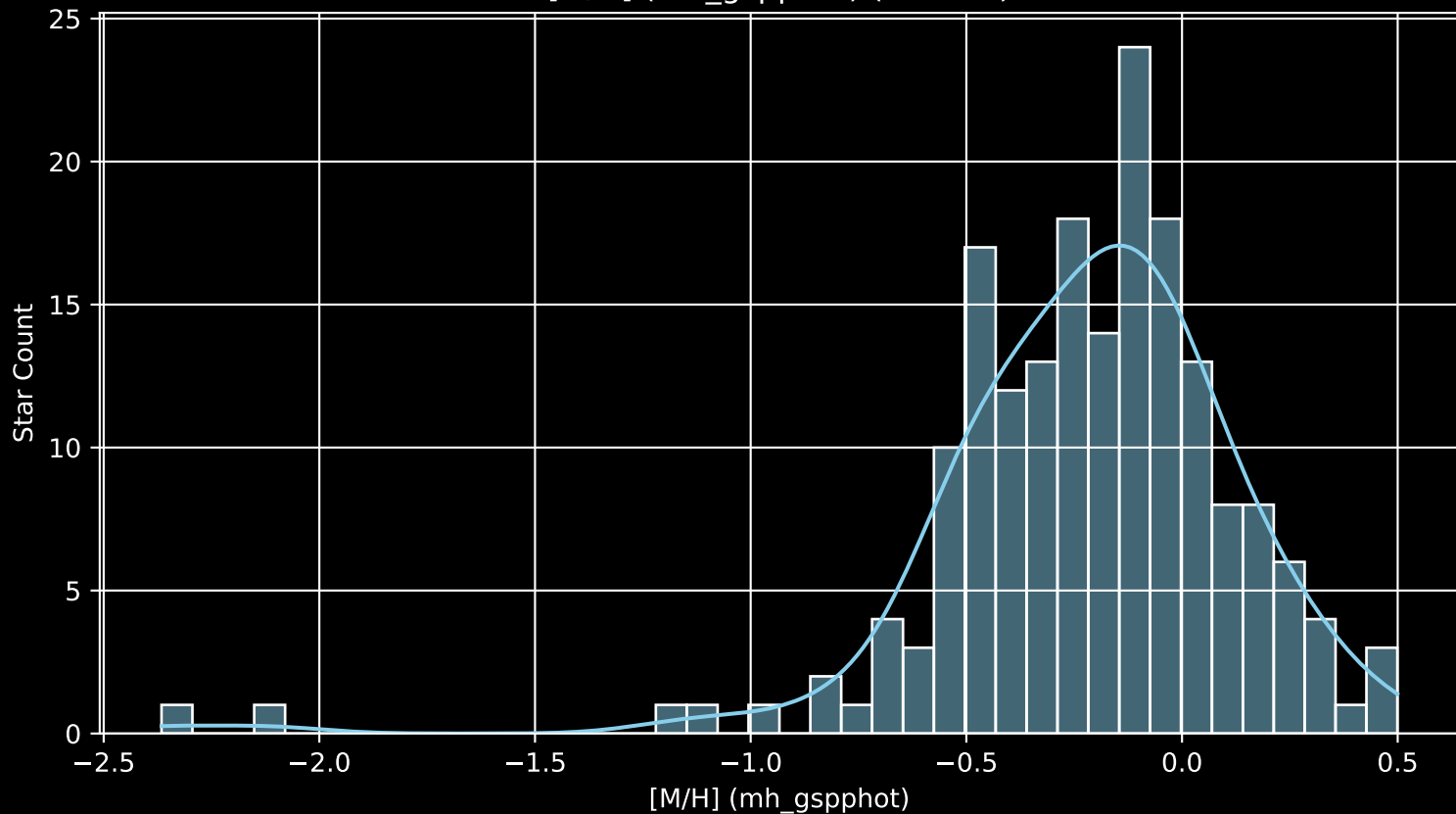
APOGEE DR17 Field: [165+62_MGA [M/H] (mh_gspphot) (n= 184)
