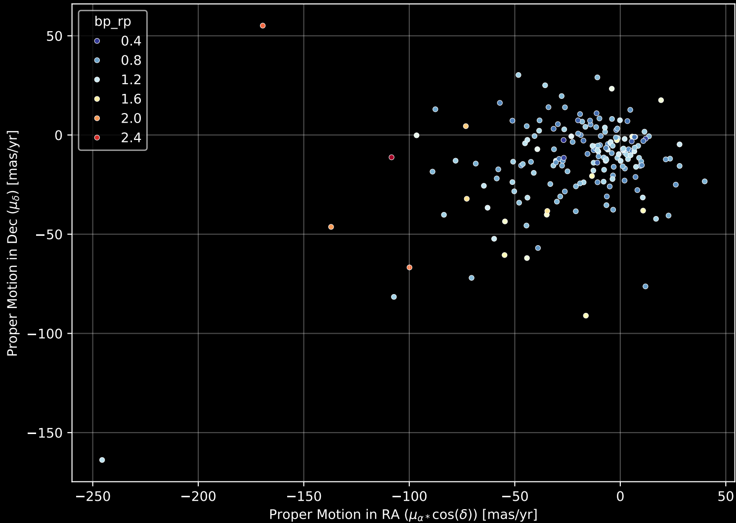
APOGEE DR17 Field: [165+62_MGA] Proper Motion Diagram (n= 184)
