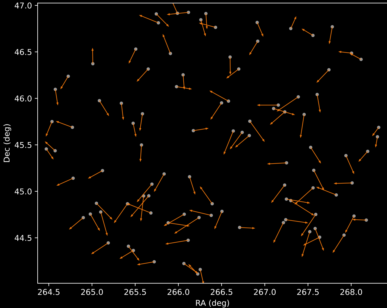
APOGEE DR17 Cluster 2 Proper Motion Vectors (n=97)
