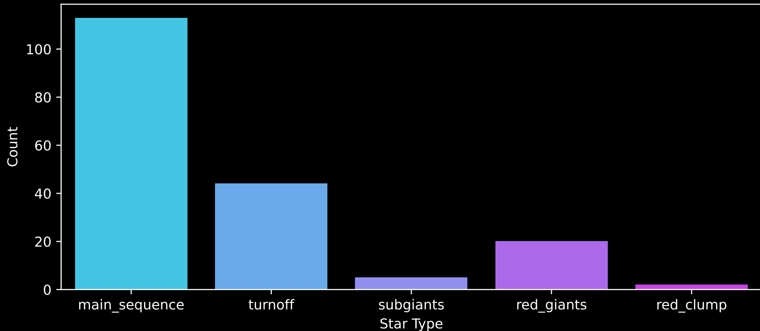
APOGEE DR17 Field: [165+62_MGA] Count plot of Star Type
